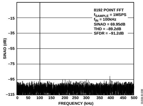
Figure 8. AD7495 Dynamic Performance
