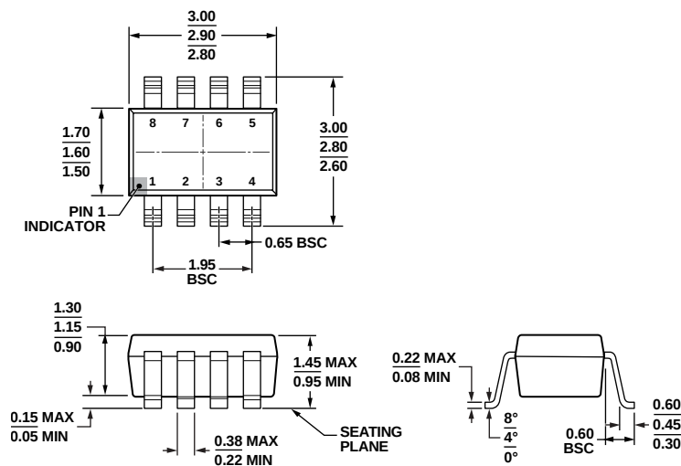
Figure 45. 8-Lead Small Outline Transistor Package [SOT-23] (RJ-8)
