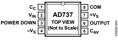
Figure 3. PDIP Pin Configuration (N-8)
