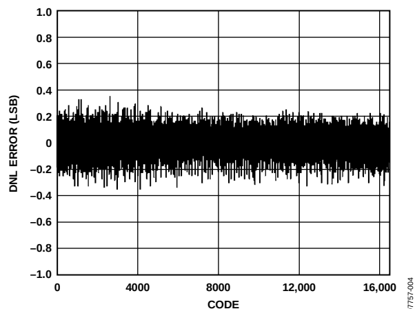
Figure 5. Typical DNL
