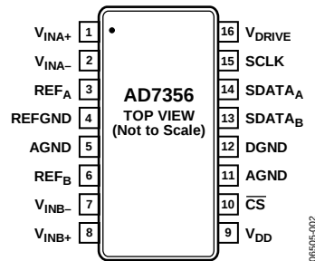
Figure 2. Pin Configuration
