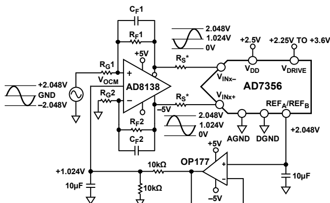
Figure 20. Using the AD8138 as a Single-Ended-to-Differential Amplifier
