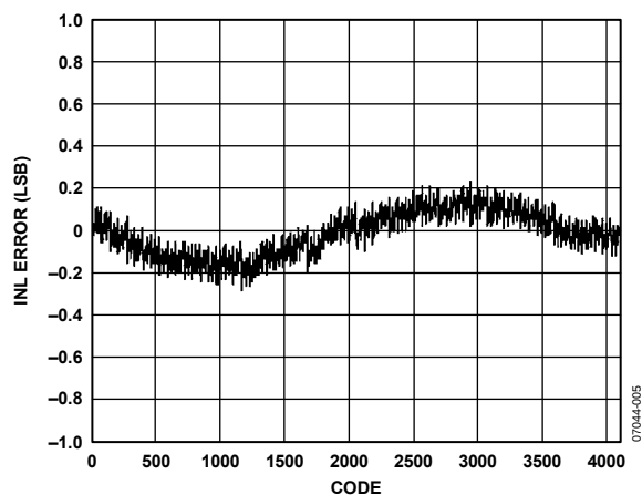
Figure 5. Typical INL Error
