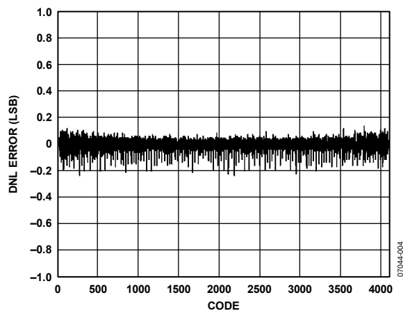
Figure 4. Typical DNL Error
