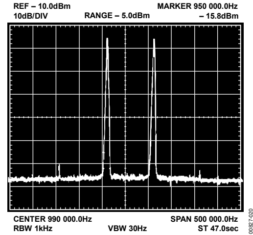
Figure 37. AD734 Third-Order Intermodulation Performance for f_1 = 9.95 MHz, f_2 = 10.05 MHz, and f_0 = 9.00 MHz and for Signal Levels of f_1 = f_2 = 6 dBm and f_0 = +24 dBm (All Displayed Signal Levels Are Attenuated 20 dB by the 10X Probe Used to Measure the Mixer's Output)
