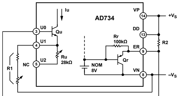
Figure 23. Connections for a Fixed Denominator
