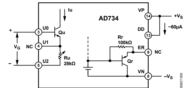
Figure 22. Low Accuracy Denominator Control
