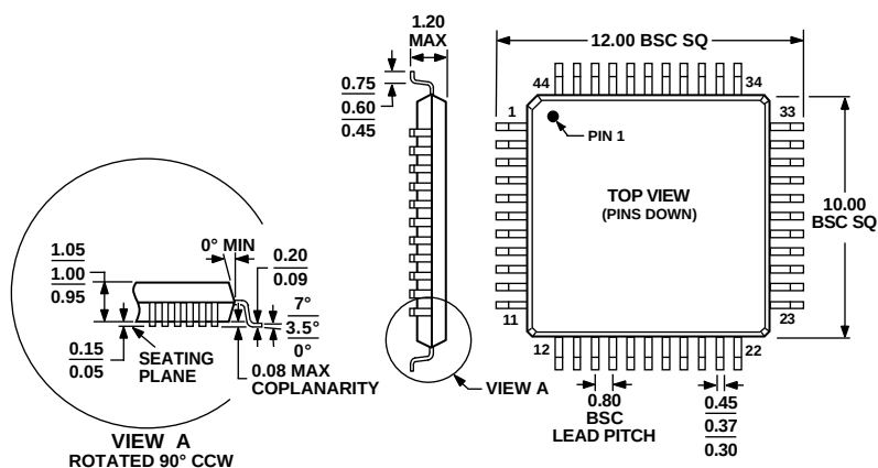
Figure 37. 44-Lead Thin Plastic Quad Flat Package [TQFP]
