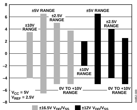
Figure 40. Pseudo Differential Input Range with V_{CC} = 5V
