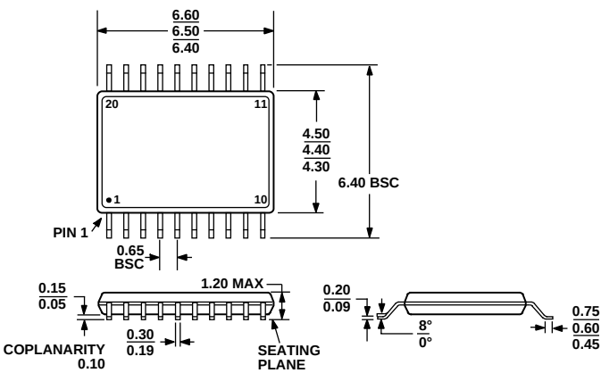
COMPLIANT TO JEDEC STANDARDS MO-153-AC Figure 57. 20-Lead Thin Shrink Small Outline Package [TSSOP] (RU-20) Dimensions shown in millimeters
