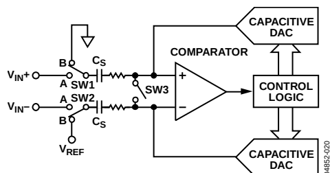
Figure 26. ADC Configuration During Conversion Phase, Differential Mode
