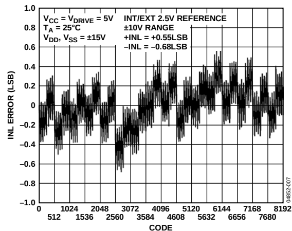
Figure 7. Typical INL for True Differential Mode
