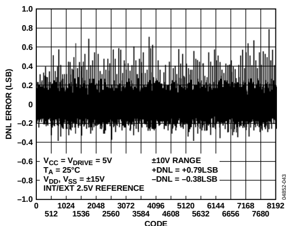
Figure 8. Typical DNL for Single-Ended Mode
