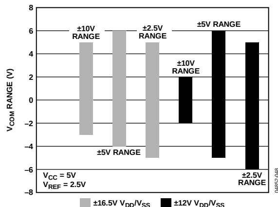
Figure 38. Common-Mode Range for V_{CC} = 5\text{ V} and V_{REF}/OUT = 2.5\text{ V}
