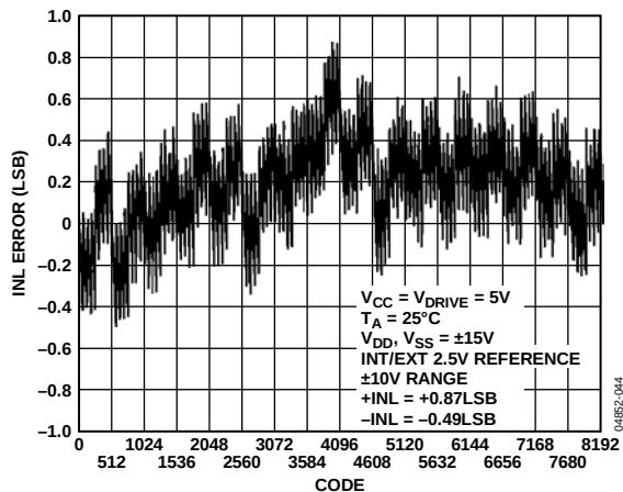
Figure 9. Typical INL for Single-Ended Mode
