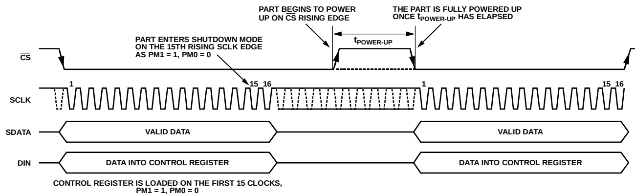
Figure 50. Entering Autoshootdown/Autostandby Mode
