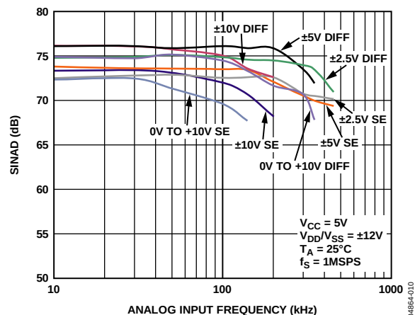
Figure 12. SINAD vs. Analog Input Frequency for Single-Ended (SE) and Differential Mode (Diff) at 5 V_{CC}
