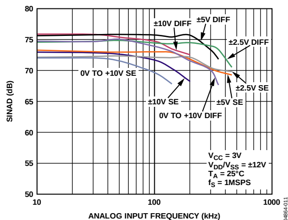
Figure 13. SINAD vs. Analog Input Frequency for Single-Ended (SE) and Differential Mode (Diff) at 3 V_{CC}
