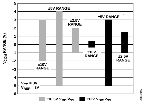
Figure 35. Common-Mode Range for V_{CC} = 3\text{ V} and REF_{IN}/OUT = 3\text{ V}
