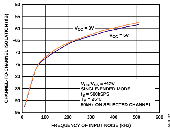
Figure 14. Channel-to-Channel Isolation
