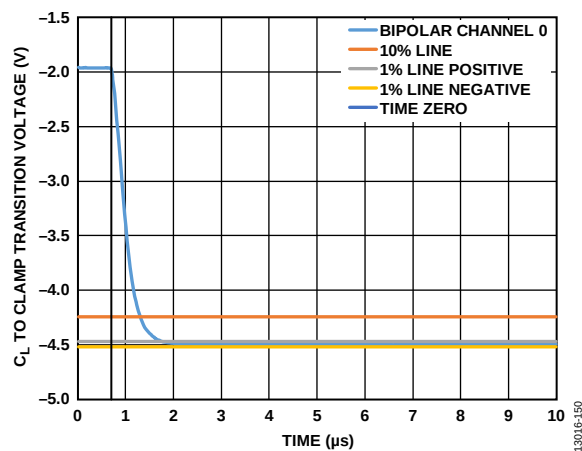
Figure 34. Closed Loop to Clamp Settling Time
