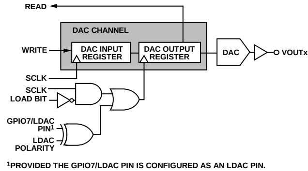
Figure 48. Simplified Diagram of Input Loading Circuitry for a Single DAC
