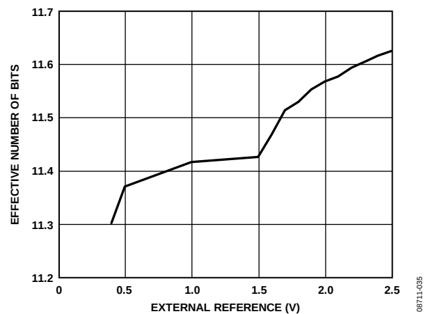
Figure 9. Effective Number of Bits vs. V_{REF} , f_{SCL} = 400kHz
