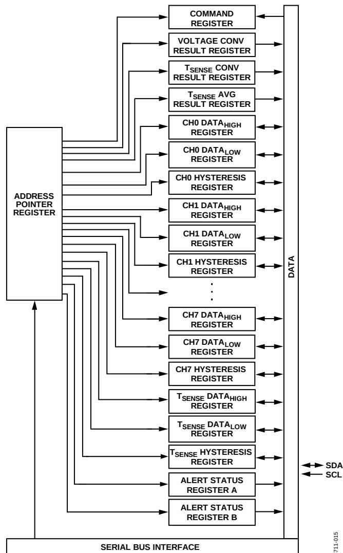
Figure 23. AD7291 Register Structure
