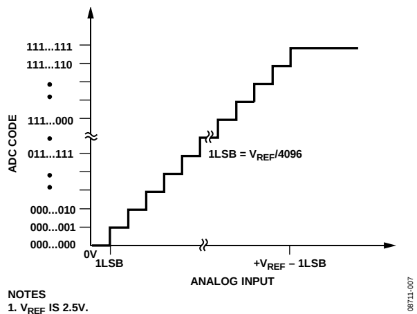
Figure 21. Straight Binary Transfer Characteristic
