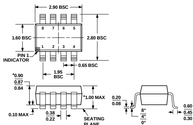
Figure 40. 8-Lead Thin Small Outline Transistor Package [TSOT] (1118)
