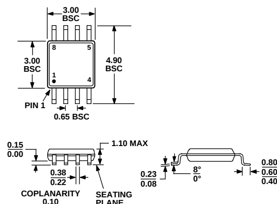
Figure 41. 8-Lead Mini Small Outline Package [MSOP] (PM 8)
