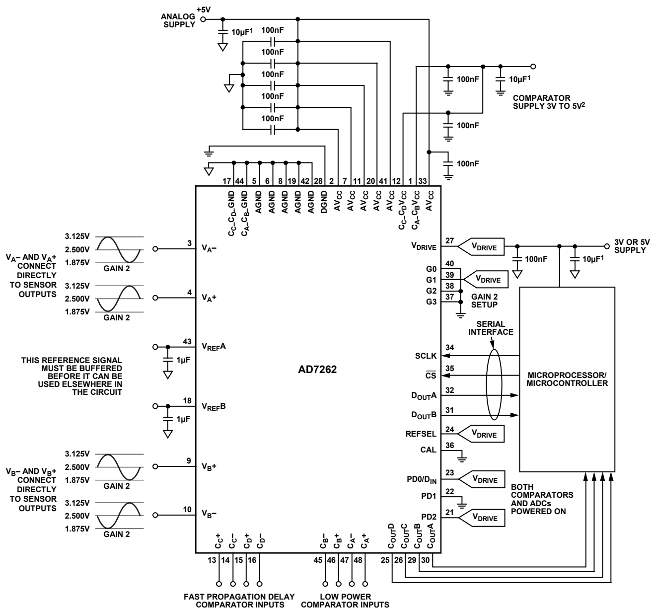
Figure 27. Typical Connection Diagram for the AD7262/AD7262-5 in Pin-Driven Mode with Gain of 2 and Both ADCs and Comparators Fully Powered On
