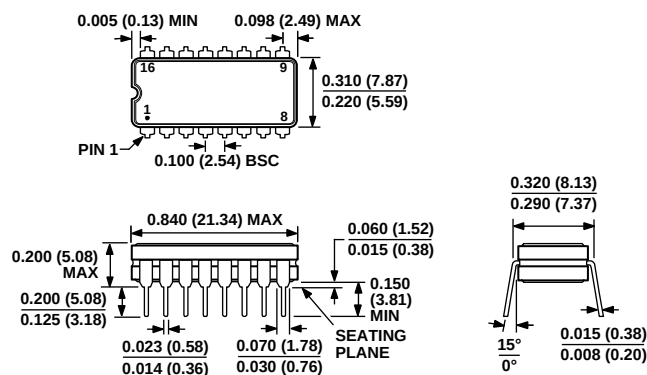
Figure 19. 16-Lead Ceramic Dual In-Line Package [CERDIP]
