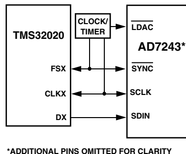
Figure 13. AD7243–TMS32020 Interface
