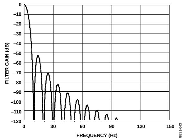
Figure 30. \text{Sinc}^4 Filter Response (FS[9:0] = 480)
