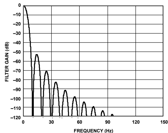
Figure 34. \text{Sinc}^4 Filter Response (FS[9:0] = 480)
