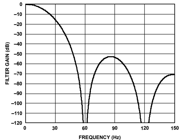
Figure 33. \text{Sinc}^4 Filter Response (FS[9:0] = 80)
