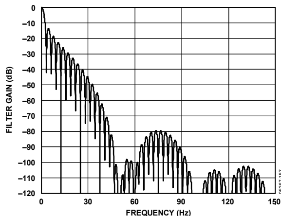
Figure 60. Filter Response for Average + Decimate Filter (Sinc 4 Filter, FS[9:0] = 96, Average by 16)
