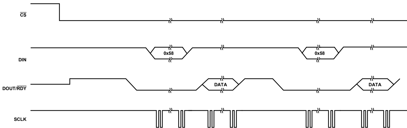
Figure 26. Continuous Conversion
