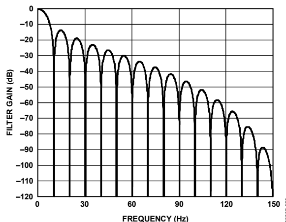
Figure 59. Filter Response for Average + Decimate Filter (Sinc 4 Filter, FS[9:0] = 30, Average by 16)
