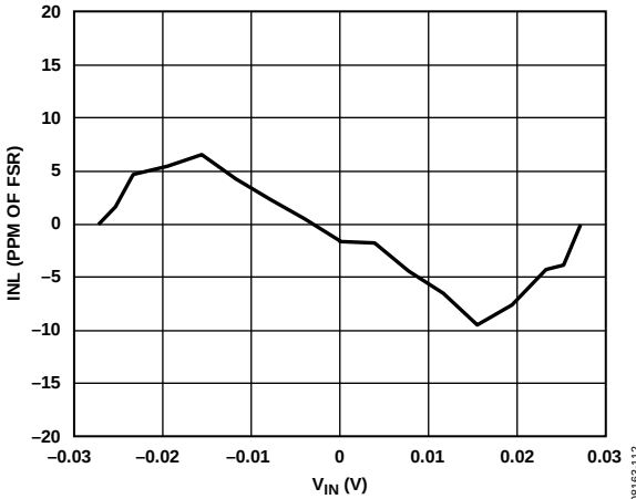
Figure 12. INL (Gain = 128)
