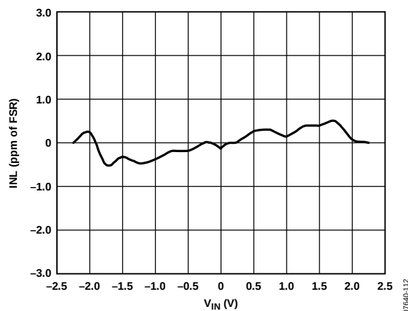
Figure 12. INL (Gain = 1)
