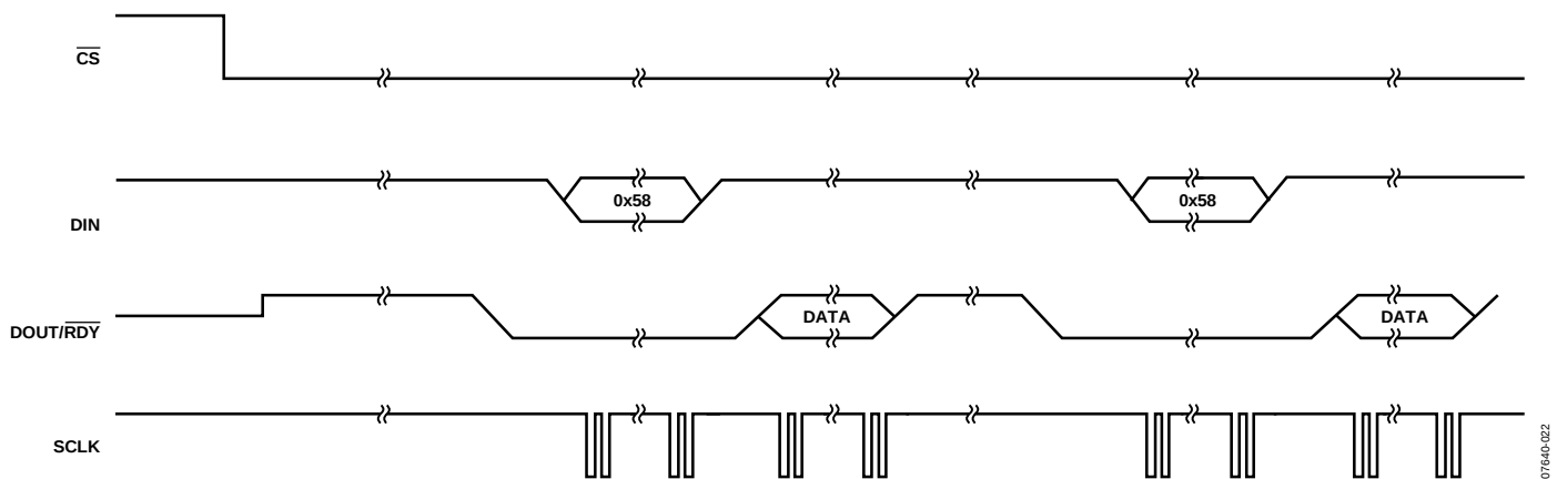
Figure 30. Continuous Conversion
