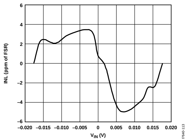
Figure 13. INL (Gain = 128)
