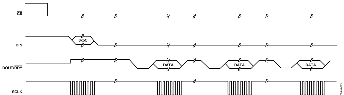
Figure 31. Continuous Read
