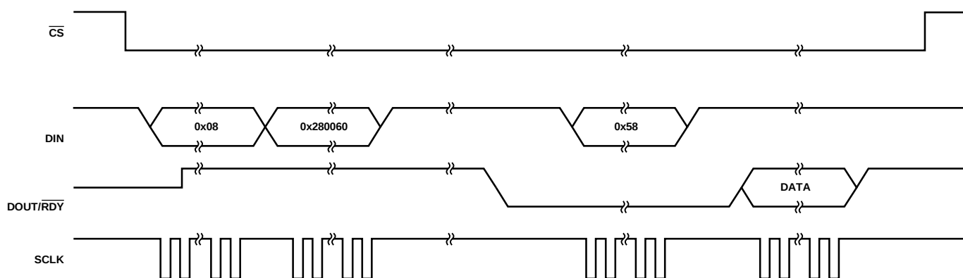
Figure 29. Single Conversion
