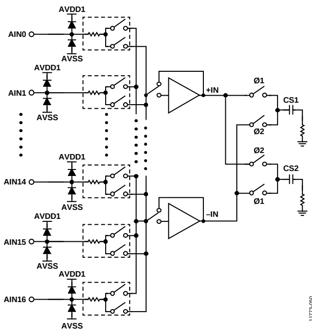
Figure 50. Simplified Analog Input Circuit
