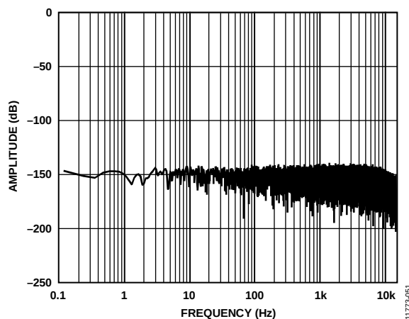
Figure 51. Shorted Input FFT
