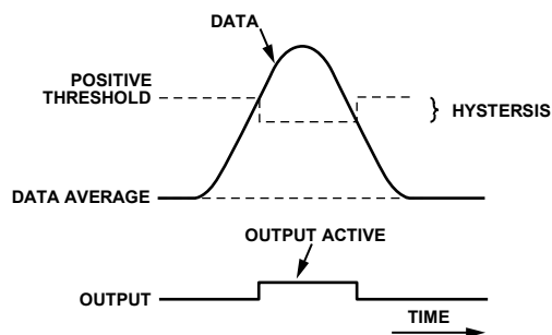
Figure 30. Threshold Hysteresis
