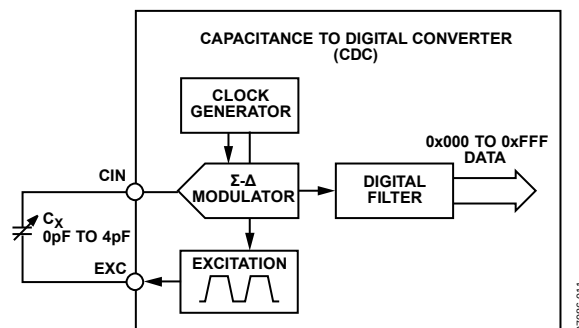
Figure 21. CDC Simplified Block Diagram
