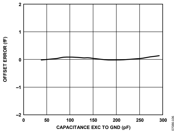
Figure 6. Capacitance Input Offset Error vs. Capacitance EXC to GND, V_{DD} = 3.3 V, CIN Pin Open Circuit
