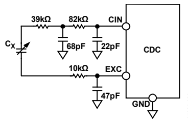
Figure 47. AD7151 CIN EMC Protection
