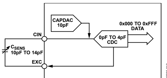
Figure 22. Using CAPDAC
