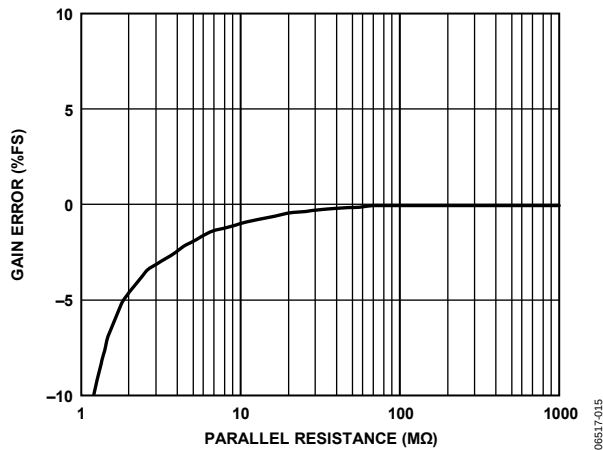
Figure 15. Capacitance Input Gain Error vs. Parallel Resistance, V_{DD} = 3.3 V, CIN to EXC = 2 pF
