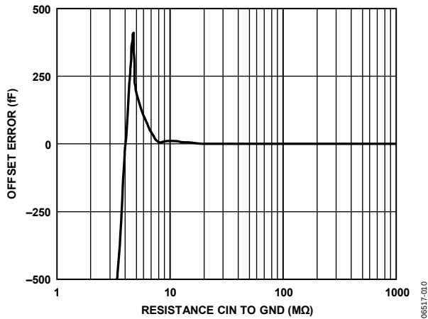
Figure 10. Capacitance Input Offset Error vs. Resistance CIN to GND, V_{DD} = 3.3 V, EXC Pin Open Circuit
