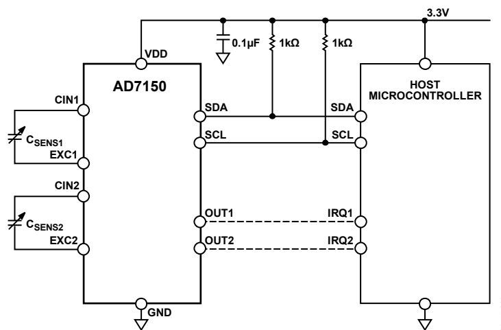
Figure 52. AD7150 Interfaced to a Host Microcontroller
