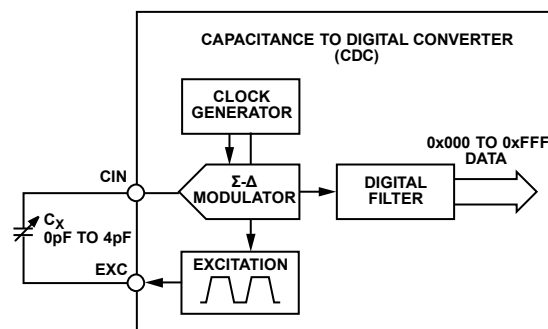
Figure 23. CDC Simplified Block Diagram
