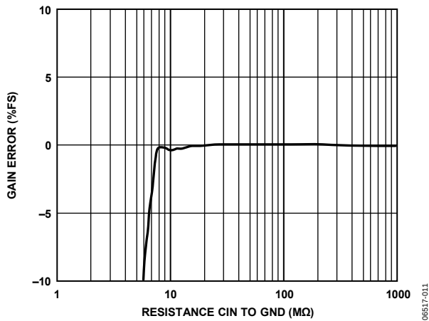
Figure 11. Capacitance Input Gain Error vs. Resistance CIN to GND, V_{DD} = 3.3 V, CIN to EXC = 2 pF
