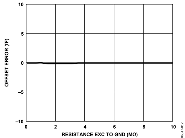
Figure 12. Capacitance Input Offset Error vs. Resistance EXC to GND, V_{DD} = 3.3 V, CIN Pin Open Circuit
