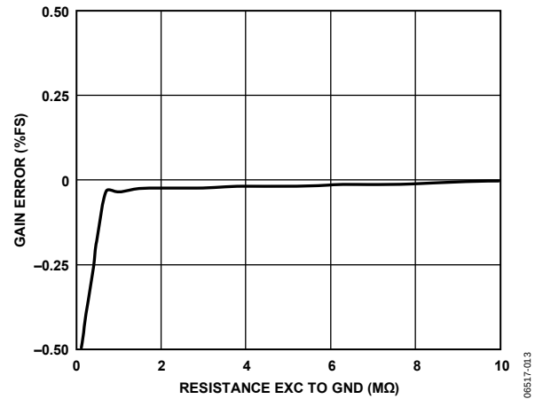
Figure 13. Capacitance Input Gain Error vs. Resistance EXC to GND, V_{DD} = 3.3 V, CIN to EXC = 2 pF
