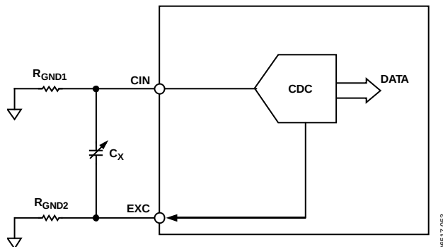
Figure 45. Parasitic Resistance to Ground
