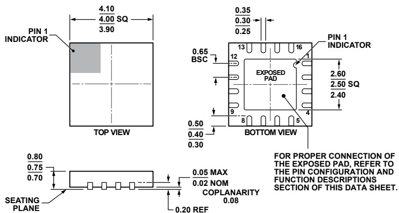
Figure 47. 16-Lead Frame Chip Scale Package [LF CSP_WQ] 4 mm x 4 mm Very Very Thin Quad (CP-16-26) Dimensions shown in millimeters
