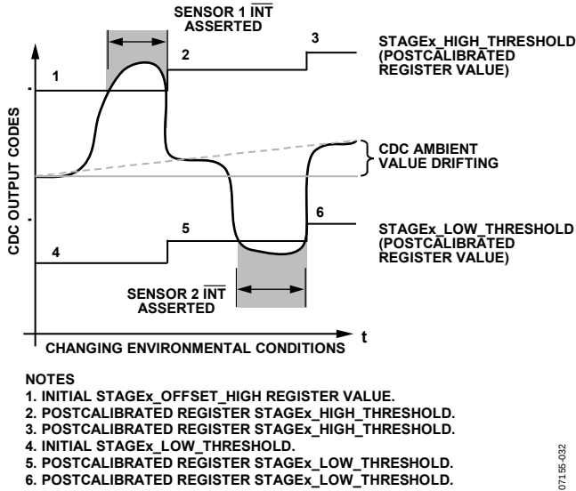
Figure 33. Typical Sensor Behavior with Calibration Applied on the Data Path
