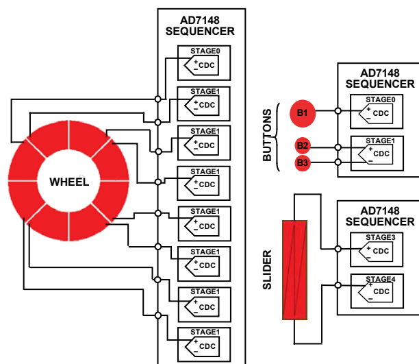
Figure 22. Sequencer Setup for Sensors
