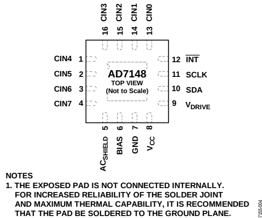
Figure 4. Pin Configuration
