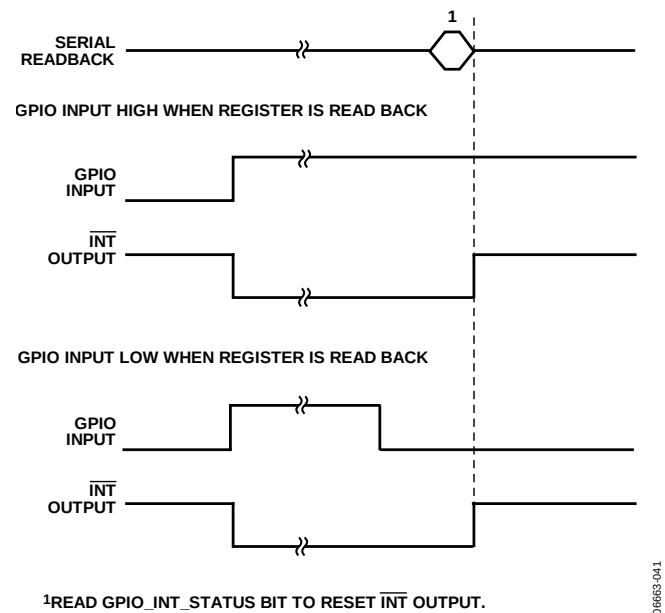
Figure 44. Example of \overline{\text{INT}} Output Controlled by the GPIO Input (GPIO_SETUP = 01, GPIO_INPUT_CONFIG = 01)
