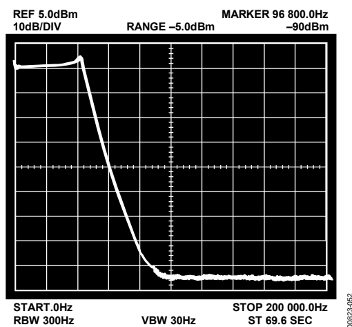
Figure 52. High Frequency Response for 9-Pole Chebyshev Filter
