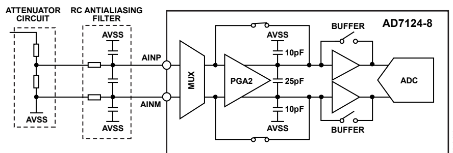
Figure 76. Input Schematic
