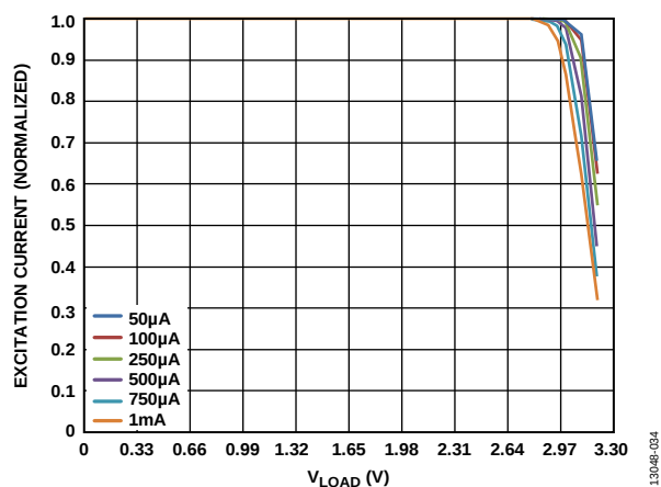
Figure 34. Output Compliance ( AV_{DD} = 3.3 V)
