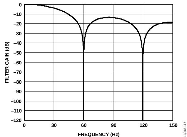
Figure 110. 60 Hz Rejection
