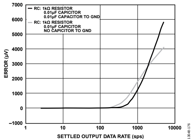
Figure 75. Error vs. Settled Output Data Rate (47 kΩ Resistors in Attenuator Circuit)
