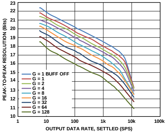
Figure 52. Peak-to-Peak Resolution vs. Output Data Rate (Settled), \text{Sinc}^4 Filter (Mid Power Mode)
