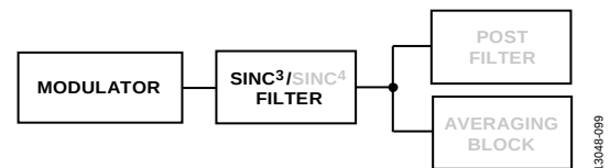
Figure 92. Sinc 3 Filter
