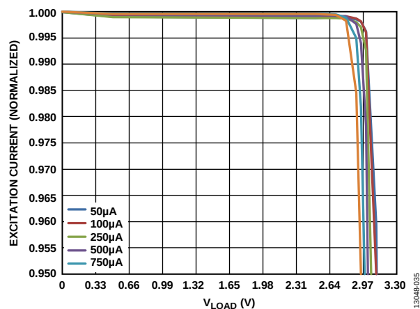
Figure 35. Output Compliance ( AV_{DD} = 3.3 V)
