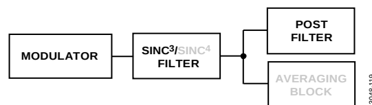
Figure 112. Post Filters
