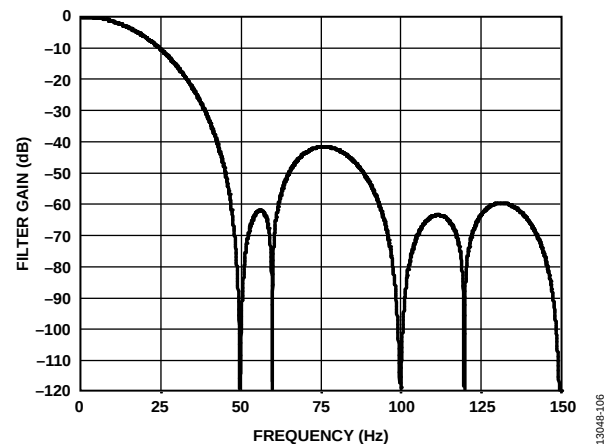
Figure 99. Sinc 3 Filter Response (50 SPS Output Data Rate, Zero Latency Disabled or 16.67 SPS Output Data Rate, Zero Latency Enabled, REJ60 = 1)
