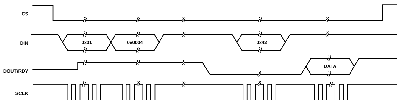
Figure 81. Single Conversion Configuration
