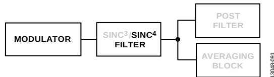
Figure 84. Sinc 4 Filter
