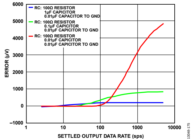
Figure 74. Error vs. Settled Output Data Rate (100 kΩ Resistors in Attenuator Circuit)
