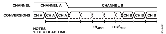
Figure 85. Sinc 4 Channel Change
