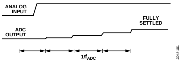
Figure 94. Asynchronous Step Change in the Analog Input
