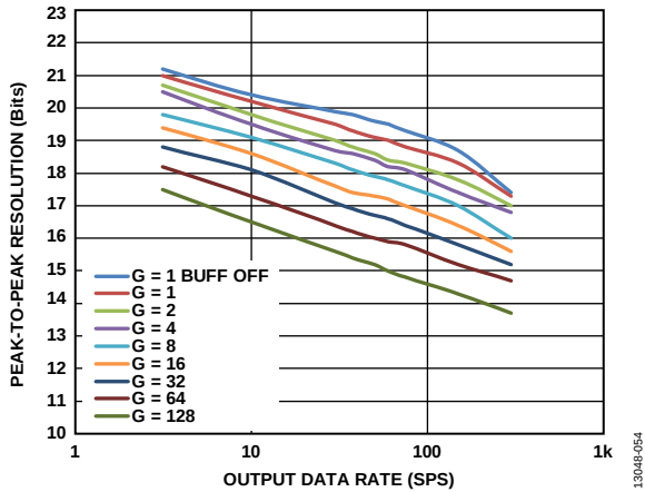
Figure 54. Peak-to-Peak Resolution vs. Output Data Rate (Settled), \text{Sinc}^4 + \text{Sinc}^1 Filter (Mid Power Mode)
