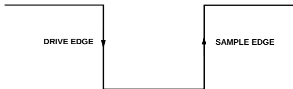
Figure 65. SPI Mode 3, SCLK Edges
