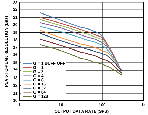
Figure 55. Peak-to-Peak Resolution vs. Output Data Rate (Settled), \text{Sinc}^3 + \text{Sinc}^1 Filter (Mid Power Mode)
