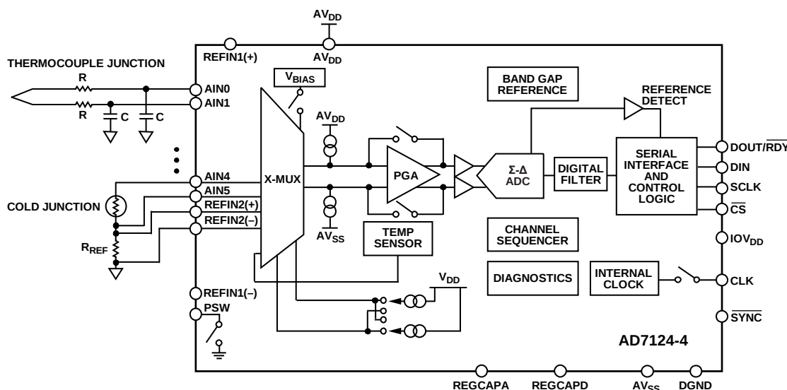
Figure 130. Thermocouple Application
