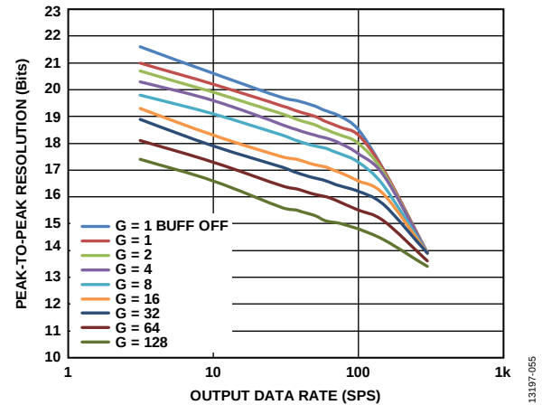
Figure 56. Peak-to-Peak Resolution vs. Output Data Rate (Settled), \text{Sinc}^3 + \text{Sinc}^1 Filter (Mid Power Mode)
