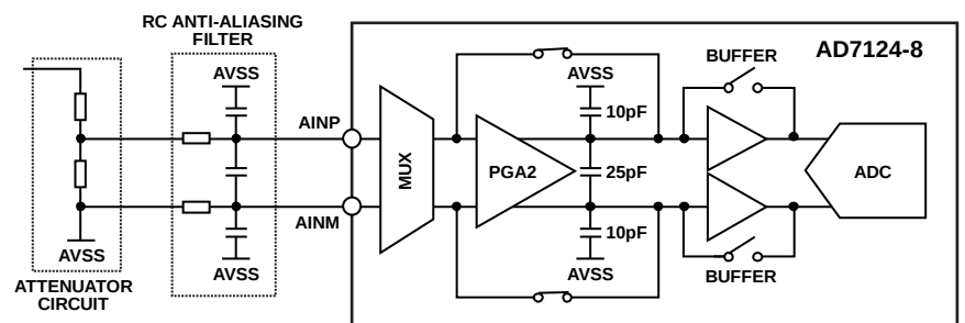
Figure 77. Input Schematic
