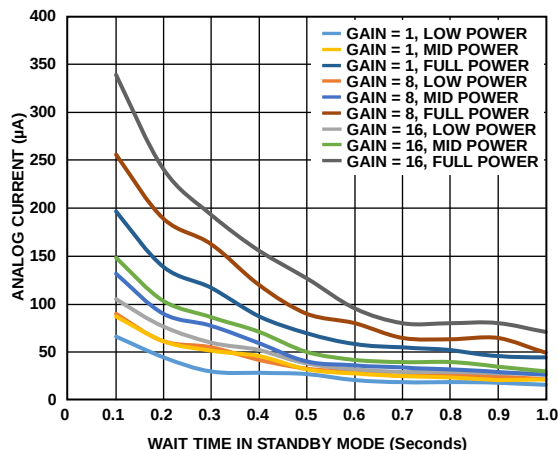
Figure 61. Analog Current vs. Wait Time in Standby Mode, ADC in Single Conversion Mode (50 SPS)
