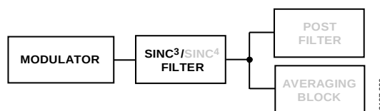
Figure 93. Sinc 3 Filter
