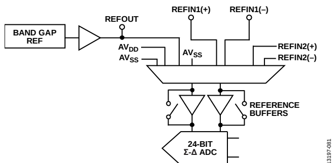
Figure 79. Reference Connections
