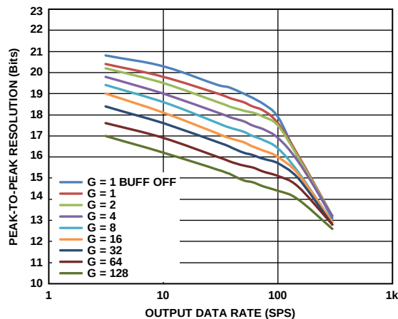
Figure 60. Peak-to-Peak Resolution vs. Output Data Rate, Sinc 3 + Sinc 1 Filter (Low Power Mode)
