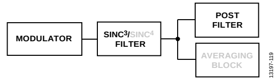
Figure 113. Post Filters
