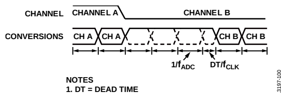
Figure 94. Sinc 3 Channel Change
