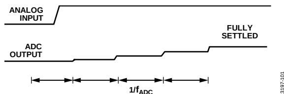
Figure 95. Asynchronous Step Change in the Analog Input
