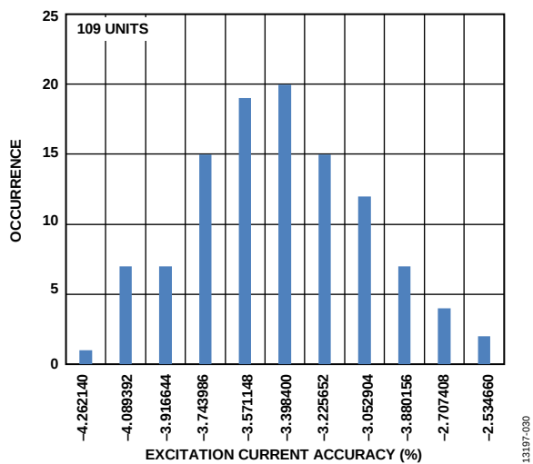
Figure 31. IOUTx Current Initial Accuracy Histogram (500 \mu A)
