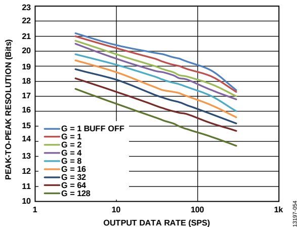
Figure 55. Peak-to-Peak Resolution vs. Output Data Rate (Settled), \text{Sinc}^4 + \text{Sinc}^1 Filter (Mid Power Mode)
