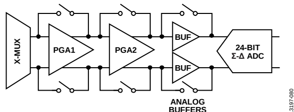
Figure 78. PGA
