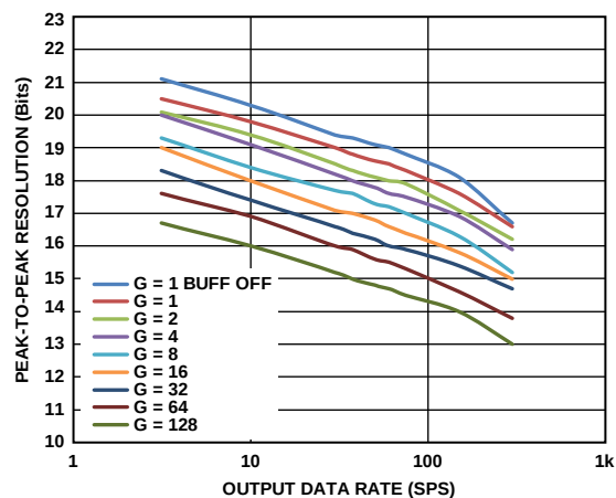
Figure 59. Peak-to-Peak Resolution vs. Output Data Rate, Sinc 4 + Sinc 1 Filter (Low Power Mode)
