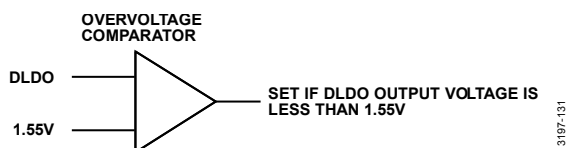
Figure 122. Digital LDO Monitor
