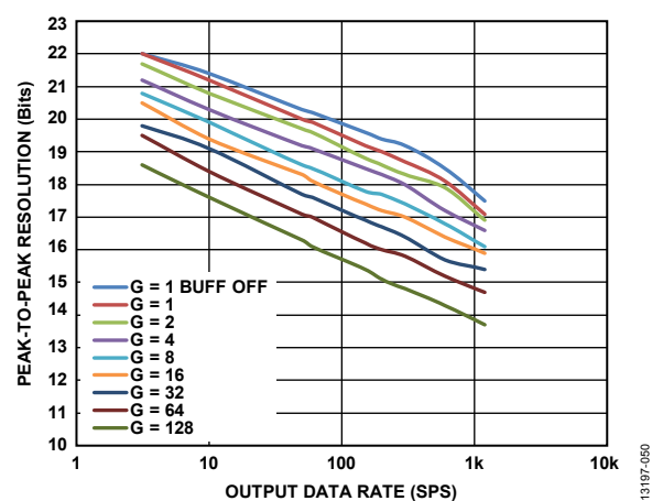
Figure 51. Peak-to-Peak Resolution vs. Output Data Rate, Sinc 4 + Sinc 1 Filter (Full Power Mode)
