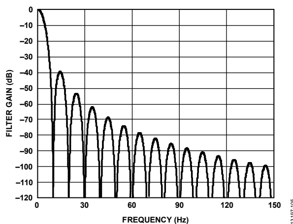
Figure 96. Sinc 3 Filter Response (10 SPS Output Data Rate, Zero Latency Disabled or 3.33 SPS Output Data Rate, Zero Latency Enabled)
