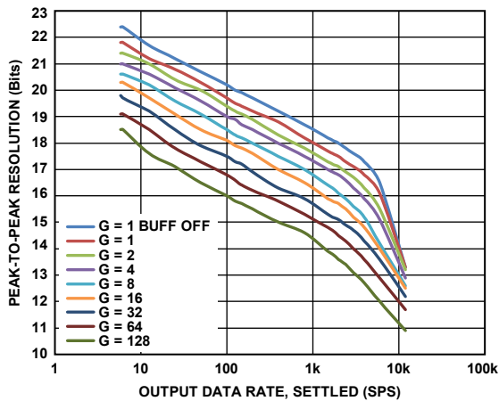
Figure 53. Peak-to-Peak Resolution vs. Output Data Rate (Settled), \text{Sinc}^4 Filter (Mid Power Mode)
