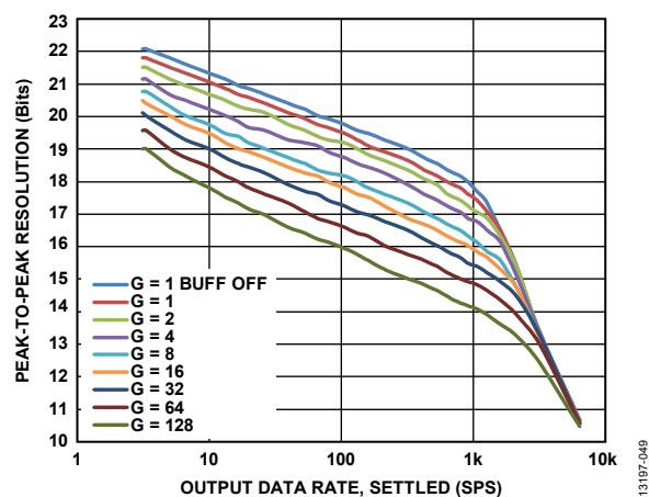
Figure 50. Peak-to-Peak Resolution vs. Output Data Rate (Settled), Sinc 3 Filter (Full Power Mode)
