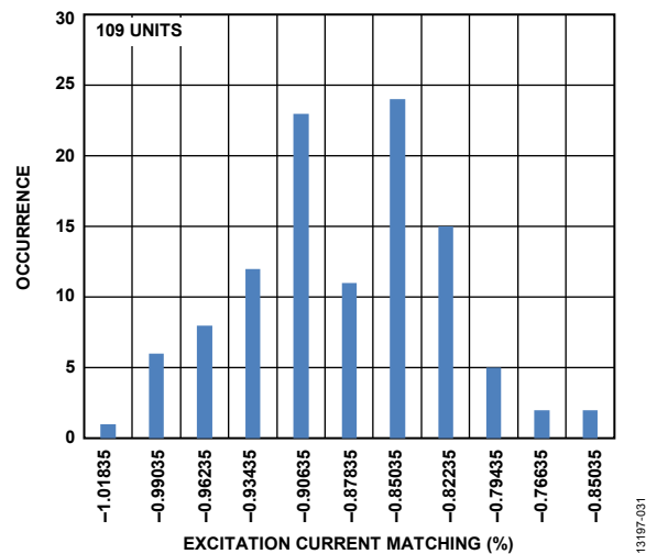
Figure 32. IOUTx Current Initial Matching Histogram (500 \mu A)
