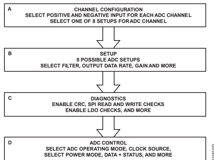
Figure 69. Suggested ADC Configuration Flow
