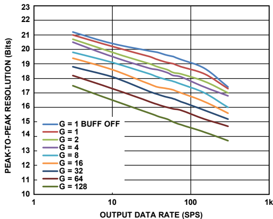
Figure 55. Peak-to-Peak Resolution vs. Output Data Rate, \text{Sinc}^4 + \text{Sinc}^1 Filter (Mid Power Mode)
