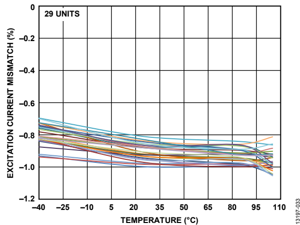
Figure 34. Excitation Current Drift Matching (500 \mu A)
