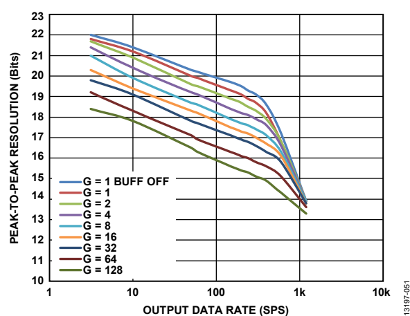
Figure 52. Peak-to-Peak Resolution vs. Output Data Rate, Sinc 3 + Sinc 1 Filter (Full Power Mode)
