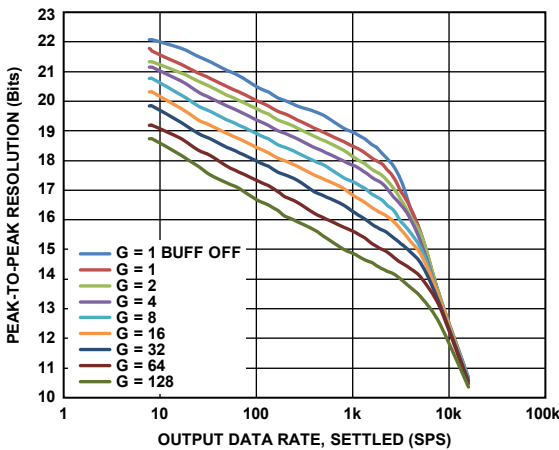
Figure 54. Peak-to-Peak Resolution vs. Output Data Rate (Settled), \text{Sinc}^3 Filter (Mid Power Mode)
