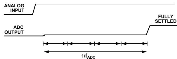
Figure 85. Sinc 4 Zero Latency Operation
