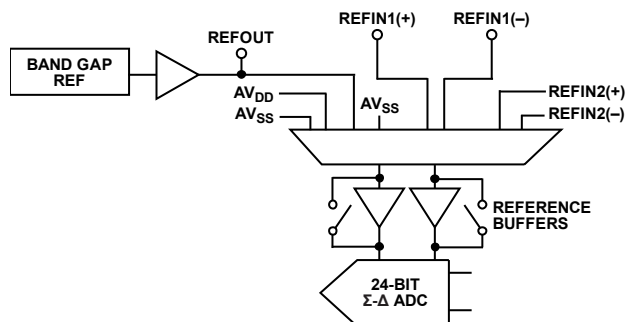
Figure 76. Reference Connections
