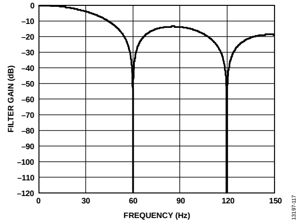
Figure 108. 60 Hz Rejection
