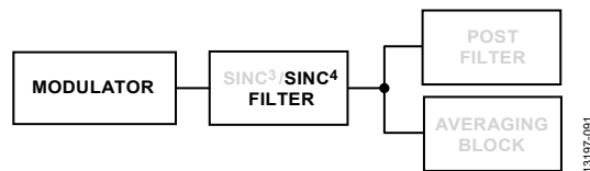
Figure 82. Sinc 4 Filter
