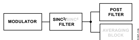
Figure 110. Post Filters
