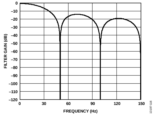
Figure 107. 50 Hz Rejection
