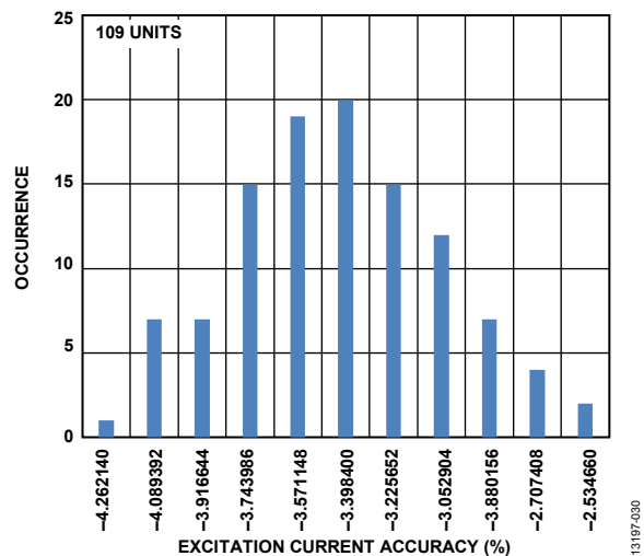
Figure 31. IOUTx Current Initial Accuracy Histogram (500 \mu A)
