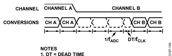
Figure 91. Sinc 3 Channel Change
