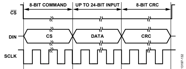
Figure 123. SPI Write Transaction with CRC
