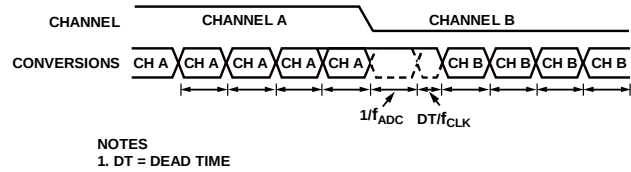
Figure 99. Fast Settling, Sinc 4 + Sinc 1 Filter
