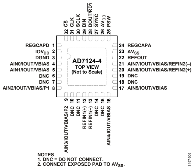
Figure 9. 32-Lead LFCSP Pin Configuration
