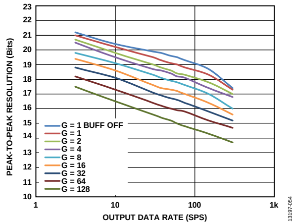
Figure 55. Peak-to-Peak Resolution vs. Output Data Rate, \text{Sinc}^4 + \text{Sinc}^1 Filter (Mid Power Mode)
