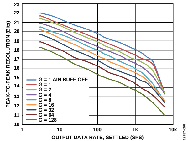
Figure 57. Peak-to-Peak Resolution vs. Output Data Rate (Settled), \text{Sinc}^4 Filter (Low Power Mode)
