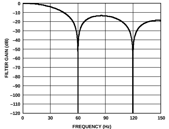
Figure 111. 60 Hz Rejection
