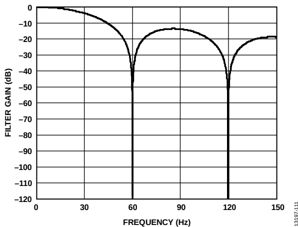
Figure 105. 60 Hz Rejection
