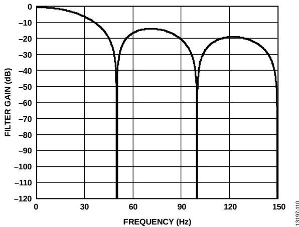
Figure 104. 50 Hz Rejection
