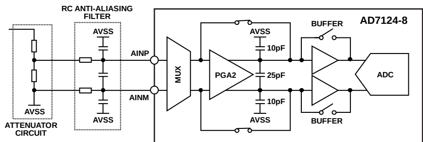
Figure 77. Input Schematic
