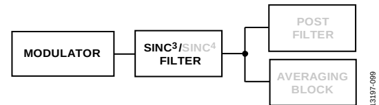
Figure 93. Sinc 3 Filter
