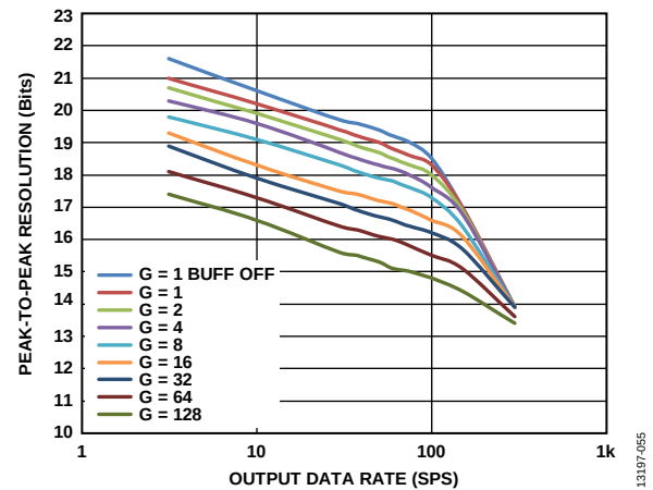
Figure 56. Peak-to-Peak Resolution vs. Output Data Rate, \text{Sinc}^3 + \text{Sinc}^1 Filter (Mid Power Mode)
