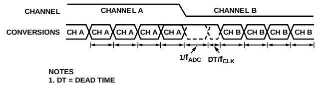
Figure 102. Fast Settling, Sinc 4 + Sinc 1 Filter
