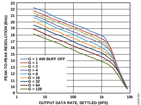
Figure 58. Peak-to-Peak Resolution vs. Output Data Rate (Settled), \text{Sinc}^3 Filter (Low Power Mode)
