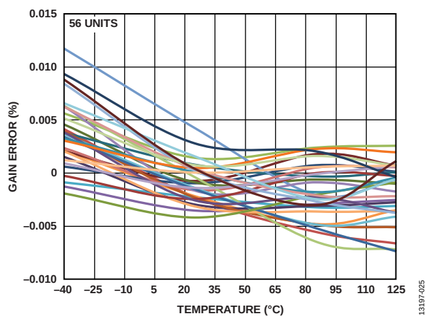
Figure 25. Input Referred Gain Error vs. Temperature (Gain = 8)
