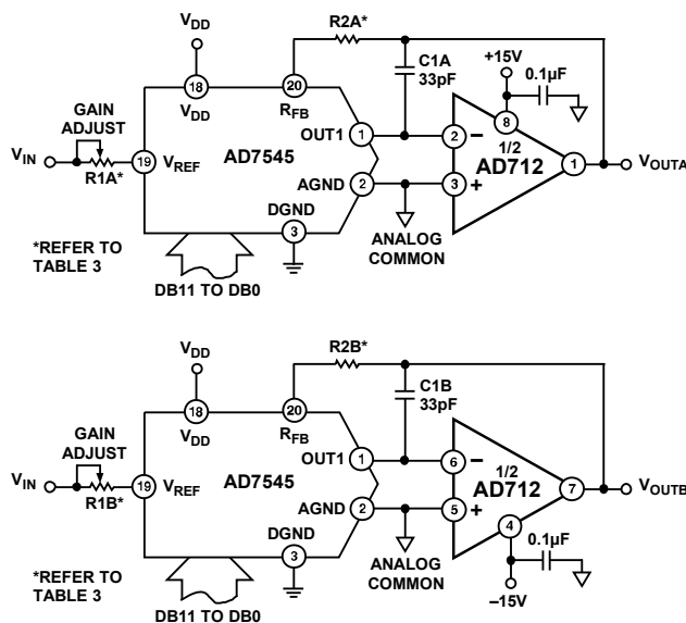
Figure 39. Unipolar Binary Operation
