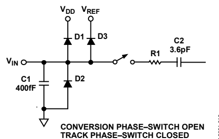
Figure 44. Equivalent Analog Input Circuit
