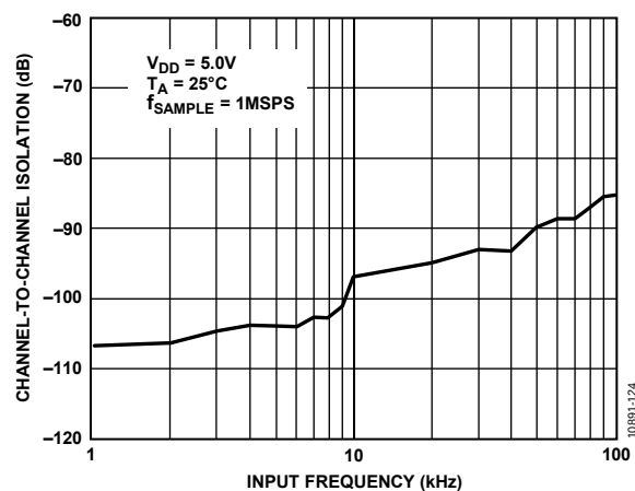
Figure 35. Channel-to-Channel Isolation vs. Input Frequency
