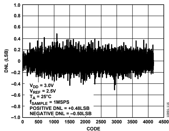
Figure 14. Differential Nonlinearity vs. Code
