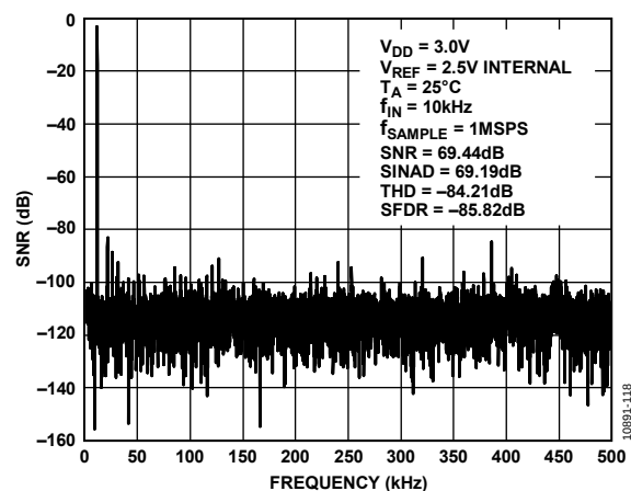
Figure 16. 10 kHz FFT, V_{DD} = 3.0\text{ V} , V_{REF} = 2.5\text{ V} Internal
