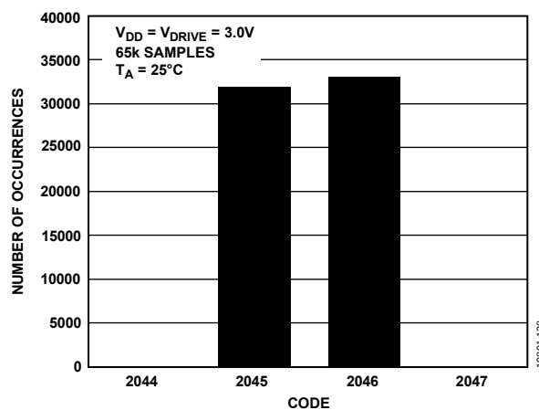
Figure 15. Histogram of a DC Input at Code Transition
