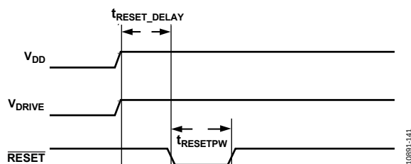
Figure 43. RESET Pin Power Up Timing
