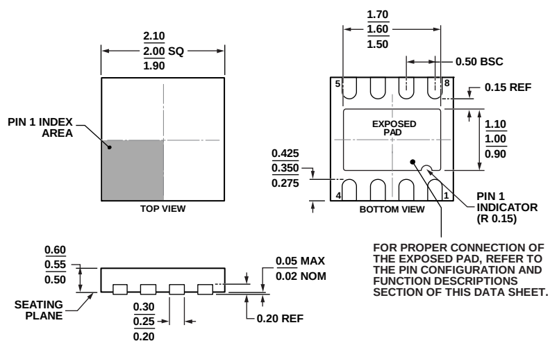
Figure 29. 8-Lead Lead Frame Chip Scale Package [LFCSP_UD] 2.00 mm × 2.00 mm Body, Ultra Thin, Dual Lead (CP-8-10)
