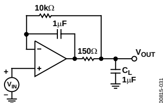
Figure 30. Compensation for Capacitive Loads
