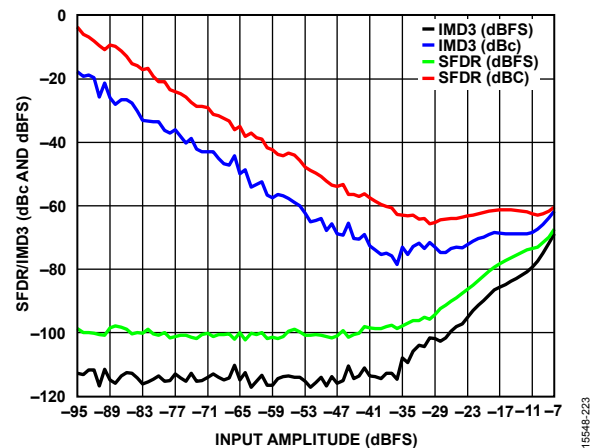
Figure 22. Two-Tone SFDR/IMD3 vs. Input Amplitude with f_{IN1} = 2137.5\text{ MHz} , f_{IN2} = 2142.5\text{ MHz}
