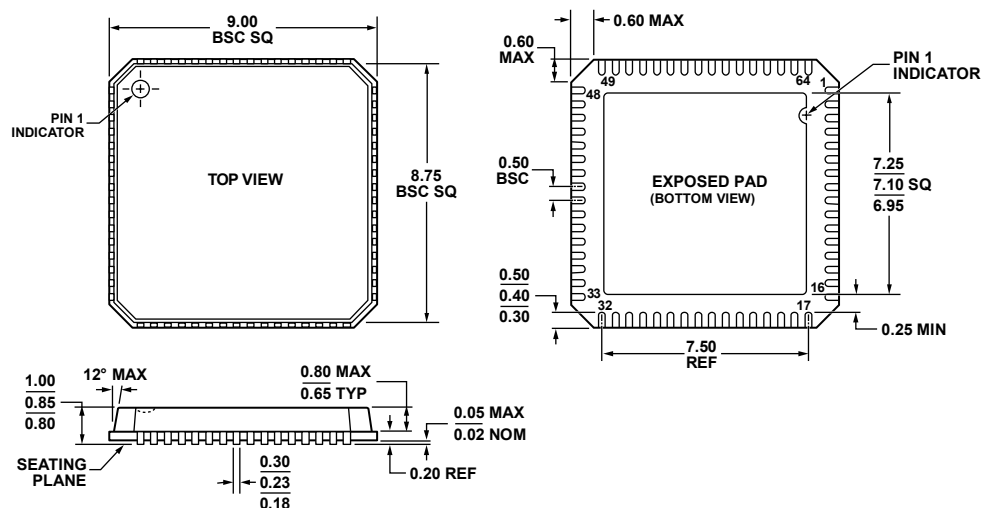
Figure 103. 64-Lead Lead Frame Chip Scale Package [LFCSP_VQ]
