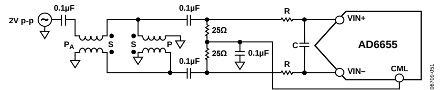
Figure 49. Differential Double Balun Input Configuration
