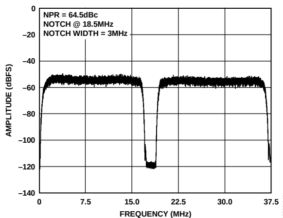
Figure 41. AD6655-150 Noise Power Ratio (NPR)
