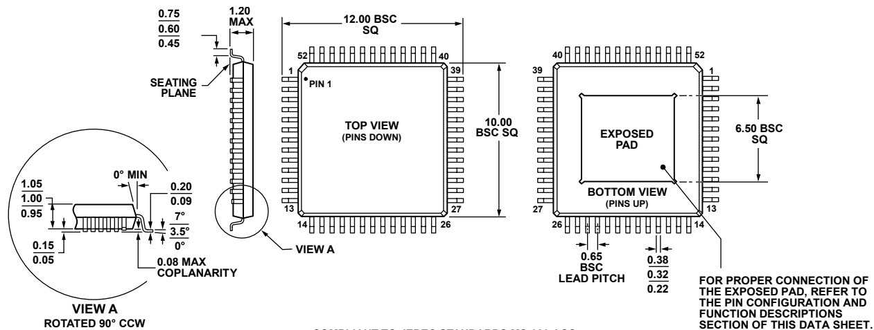
Figure 48. 52-Lead Thin Quad Flat Package, Exposed Pad [TQFP_EP] (SV-52-1)
