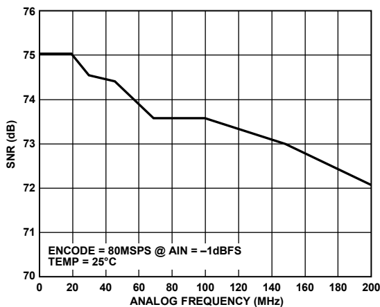
Figure 12. Signal-to-Noise Ratio (SNR) vs. Analog Frequency (fF)
