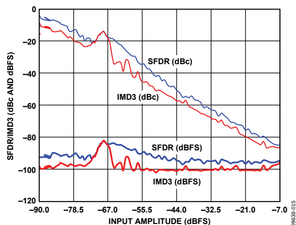
Figure 15. AD6643-200 Two Tone SFDR/IMD3 vs. Input Amplitude ( A_{IN} ) with f_{IN1} = 184.12 MHz, f_{IN2} = 187.12 MHz
