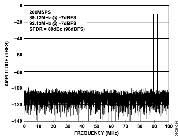
Figure 16. AD6643-200 Two Tone FFT with f_{IN1} = 89.12 MHz, f_{IN2} = 92.12 MHz
