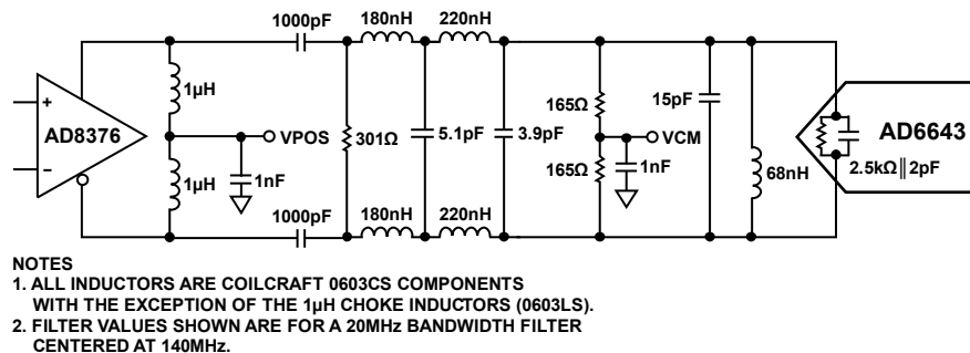
Figure 45. Differential Input Configuration Using the AD8376
