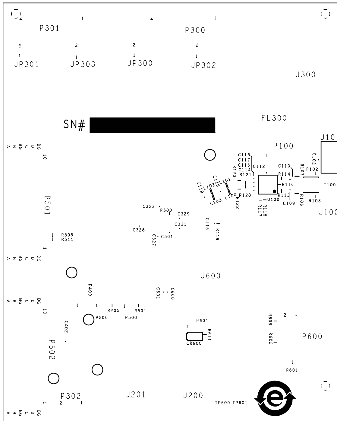
Figure 31. Bottom Silk Screen
