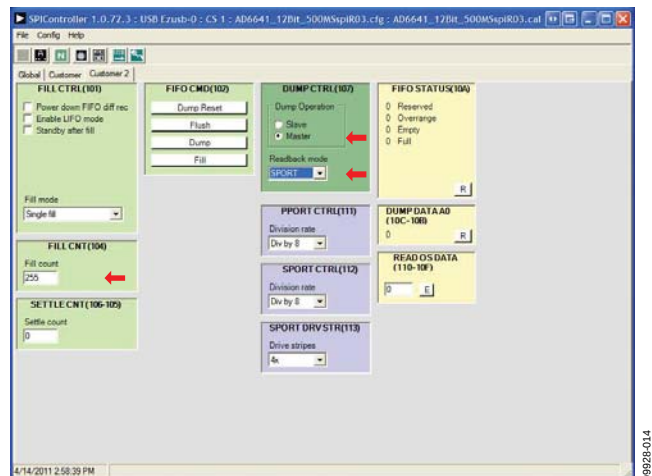
Figure 14. SPI Controller, Customer Tab
