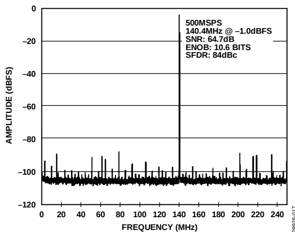
Figure 17. Typical FFT, AD9434
