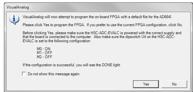
Figure 6. VisualAnalog Default Configuration Message
