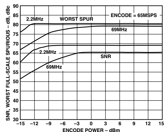
TPC 12. SNR, Worst Spurious vs. ENCODE Power
