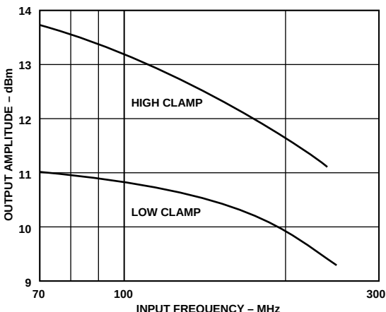
Figure 5. Clamp Level vs. Frequency
