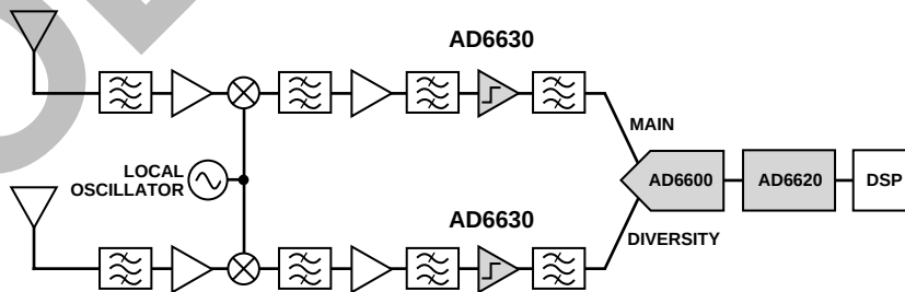
Figure 1. Reference Design
