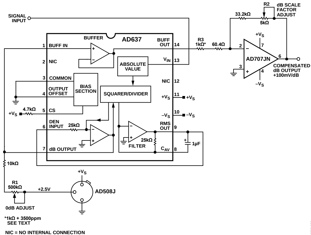
Figure 20. dB Connection
