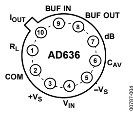
Figure 3. 10-Pin TO-100 Pin Configuration
