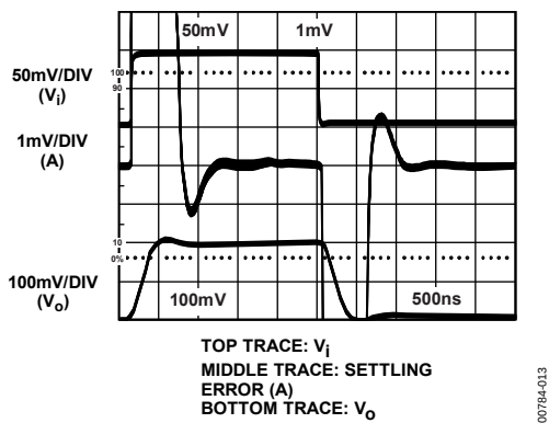
Figure 14. Small Signal Noninverting Step Response (See Figure 18)
