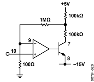
Figure 26. Comparator Hysteresis
