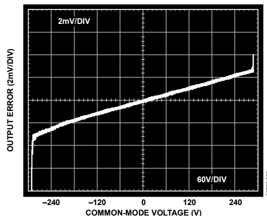
Figure 3. Error Voltage vs. Input Common-Mode Voltage
