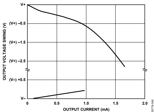
Figure 40. Output Voltage Swing vs. Output Current
