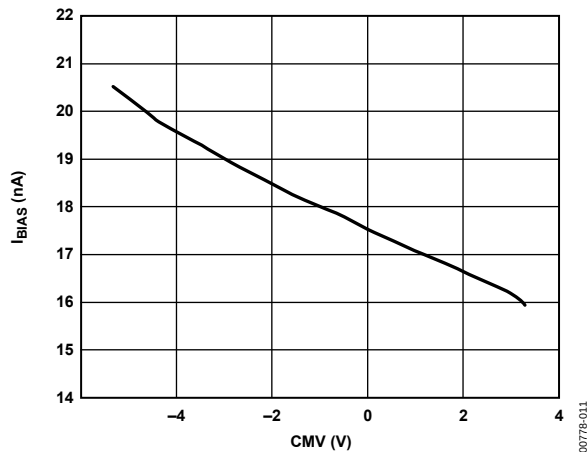
Figure 11. I_{BIAS} vs. CMV, V_S = \pm 5 V
