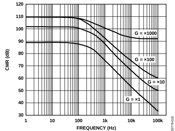
Figure 18. CMR vs. Frequency for Various Gain Settings (G)
