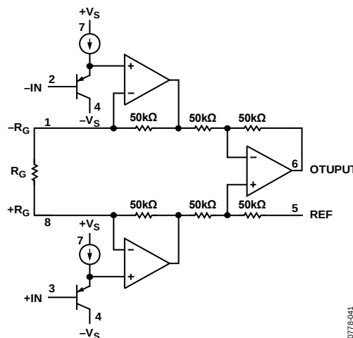
Figure 41. Simplified Schematic
