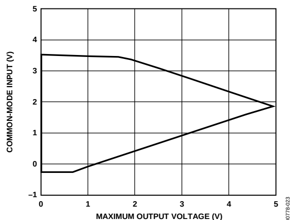
Figure 23. Maximum Output Voltage vs. Common-Mode Input, G \geq 10 , +V_S = 5 \text{ V} , -V_S = 0 \text{ V} , R_L = 100 \text{ k}\Omega
