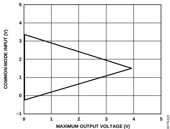
Figure 22. Maximum Output Voltage vs. Common-Mode Input, G = 1 , +V_S = 5 \text{ V} , -V_S = 0 \text{ V} , R_L = 100 \text{ k}\Omega
