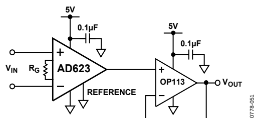
Figure 52. Output Buffering
