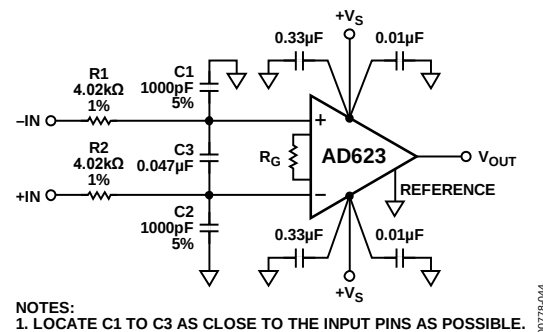
Figure 45. Circuit to Attenuate RF Interference
