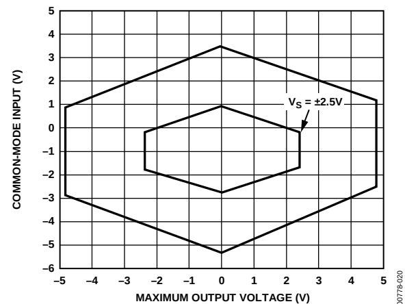
Figure 20. Maximum Output Voltage vs. Common-Mode Input, G = 1 , R_L = 100 k \Omega for Two Supply Voltages
